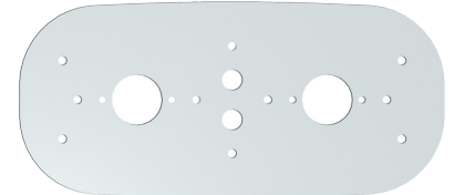
VP170107 DUAL WATERMELON INTERIOR PLATE W/2 SWITCH HOLE (389 DOME LIGHT)
